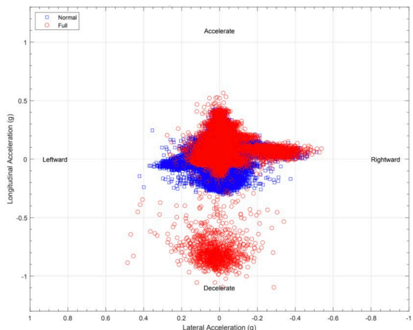
Normal versus aggressive driving accelerometer data.
