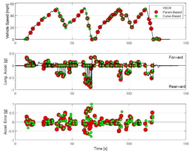
Comparison of vehicle speed, longitudinal acceleration and acceleration error in devices tested.
